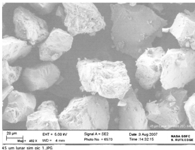
Figure 5. SEM image of JSC-1, scale bar 20 μm (Fred Minetto and Steve Curtis, NASA/GSFC)
