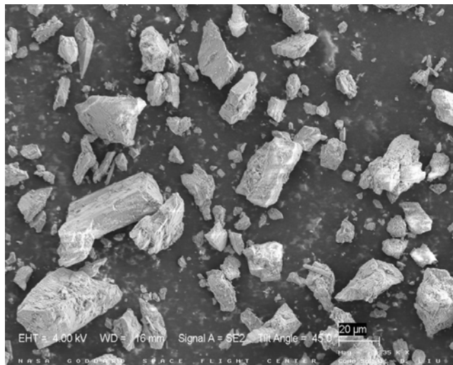
Figure 4. SEM image of GSC-1, scale bar 20 μm (Fred Minetto and Steve Curtis, NASA/GSFC)
