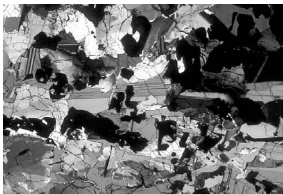
Figure 2. Lunar thin section 40X, cross polarized light (Apollo 17)-from Dr. Kurt Hollecher (Union College).
